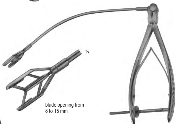
COOLEY PQ-387 Dilator for mitral valve for children
