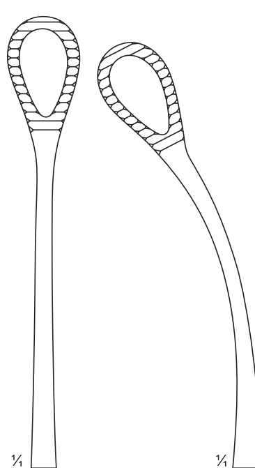
EF-018 Serrated Jaws
